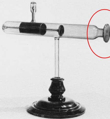
Lenard tube (1894). The tube has a perforated end piece over which gold leaf or aluminum foil could be fitted before the tube was evacuated.
